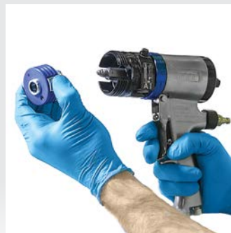
Press the new PC fluid cartridge onto the mix chamber
